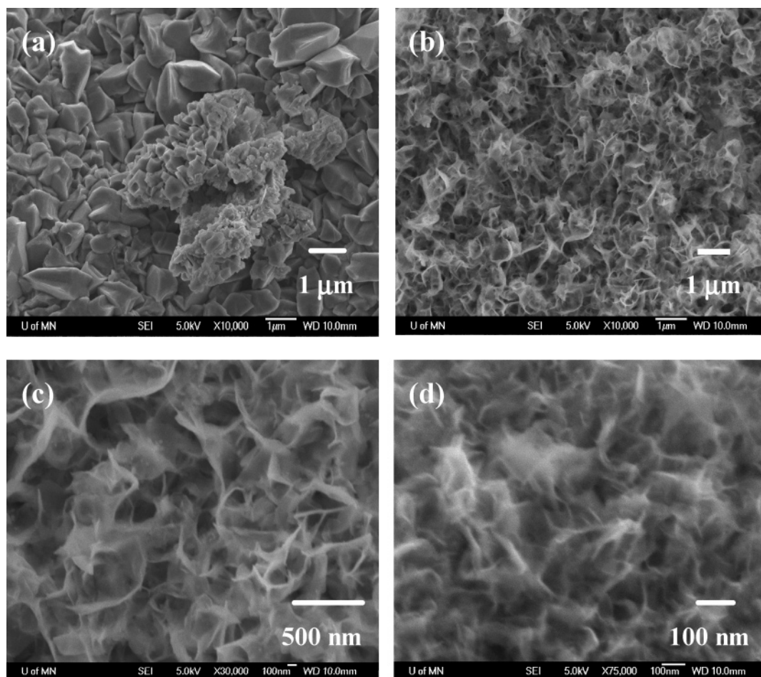
Figure 7. SEM images of samples after salt removal. (a) Sample v1 (reactant inlet velocity = 4 m/s): salt aggregates are no longer present, and there is a residue of titanium left behind in the regions where salt was removed. (b and c) Sample v2 (reactant inlet velocity = 5 m/s): highly porous film left behind after salt removal. (d) Sample v3 (reactant inlet velocity = 6 m/s).
