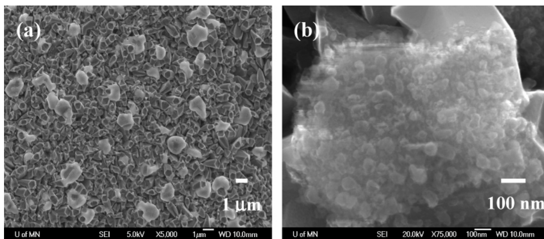
Figure 3. (a) SEM image of sample v1 (reactant inlet velocity = 4 m/s) indicates a uniform base structure with diamond-shaped crystallites of titanium, and aggregates of salt spread over the surface. (b) High magnification image of salt aggregate (acceleration voltage of electron beam = 20 kV) reveals titanium enclosed within salt matrix.
