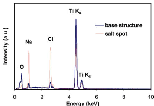
Figure 4. EDX spectra of sample v1 (reactant inlet velocity = 4 m/s) from two different regions, one on the base structure and the other on a salt aggregate.
