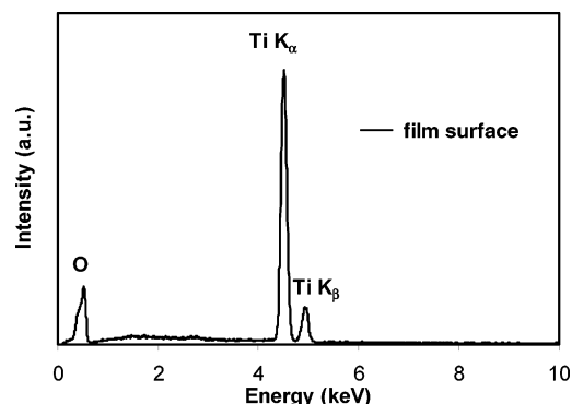
Figure 8. EDX spectrum of sample v1 (reactant inlet velocity = 4 m/s) after removal of salt shows the absence of Na and Cl and peaks for Ti and O.
