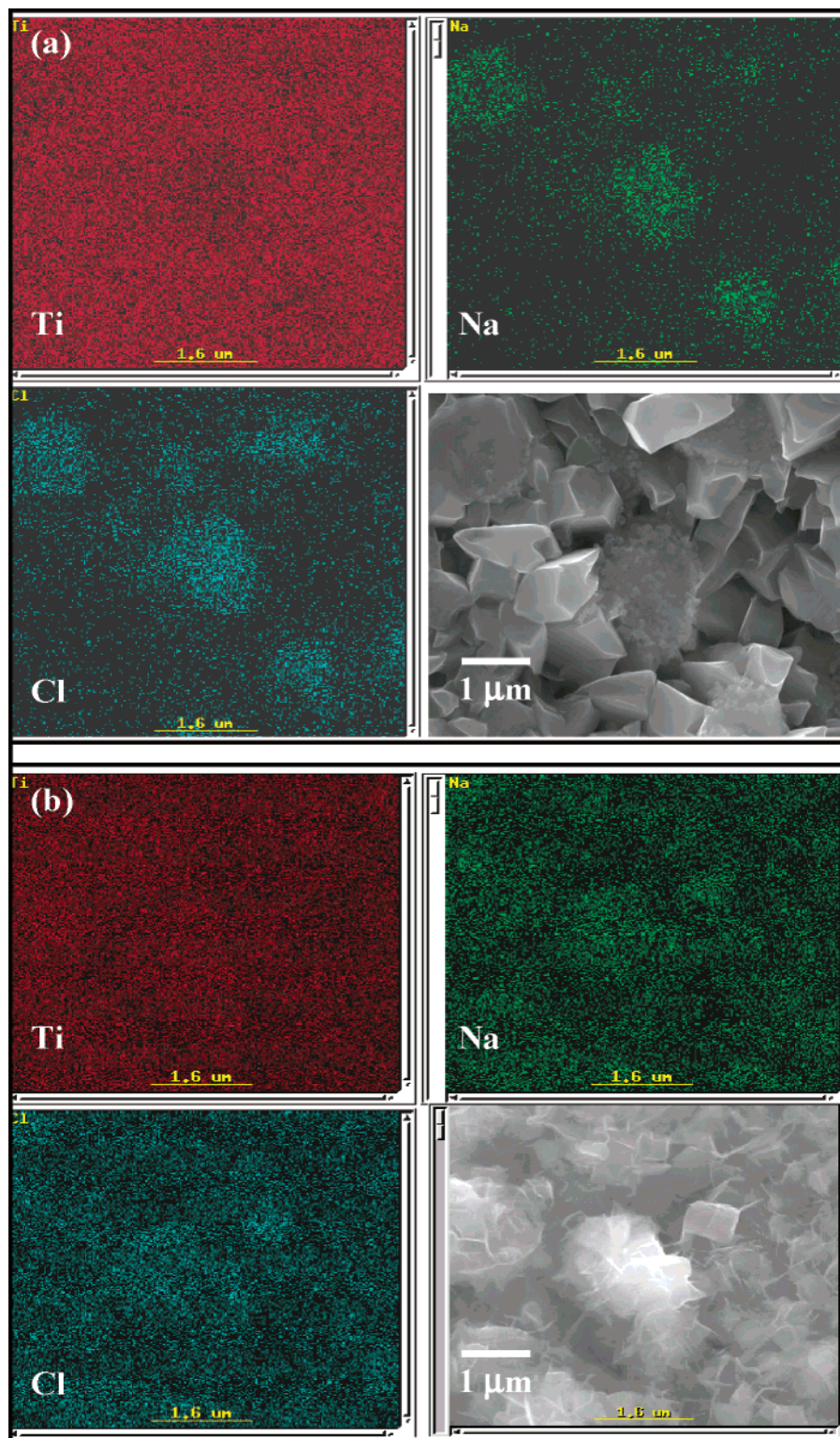
Figure 6. X-ray maps of Ti, Na, and Cl. Clockwise from bottom left, Cl, Ti, and Na SEM image; the scale bar applies for maps as well as SEM image. (a) X-ray elemental mapping for sample v1 (reactant inlet velocity = 4 m/s) shows a nearly uniform distribution of Ti over the entire surface, while Na and Cl are confined to salt aggregates. (b) Map for sample v3 (reactant inlet velocity = 6 m/s) suggests a more uniform distribution of Na and Cl over the entire substrate surface.
