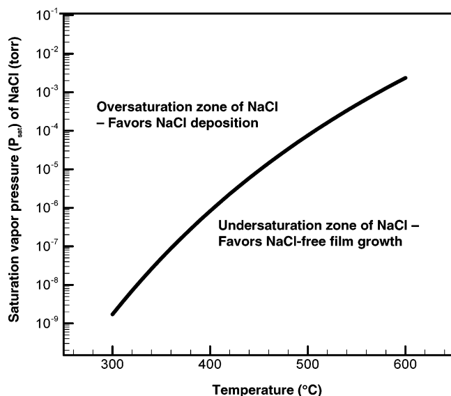
Figure 2. Variation of saturation vapor pressure of NaCl with temperature. 14
